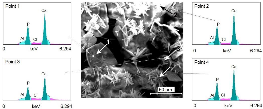
Fig. (6). EDS analysis data and SEM micrograph of the morphology of calcium phosphate coating deposited by the thermal method on a Ti6Al4V/Al 2 O 3 substrate. Left and right panels: EDS analyses of selected points. Center panel: SEM micrograph with selected points indicated.
