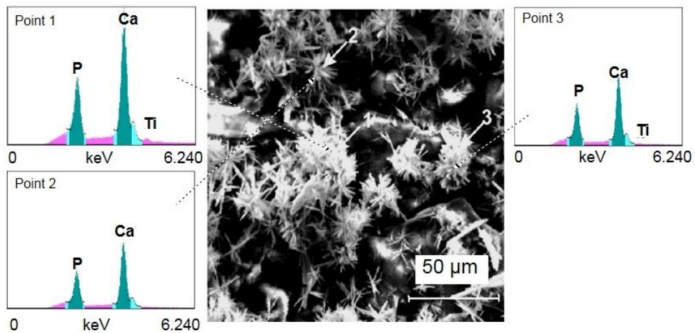
Fig. (5). EDS analyses data and SEM micrograph of the morphology of a calcium phosphate coating deposited by the thermal method on a Ti6Al4V substrate. Left and right panels: EDS analyses of selected points. Center panel: SEM micrograph with selected points indicated.
