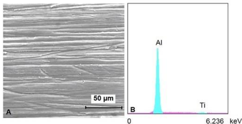
Fig. (3). (A) SEM micrograph of surface morphology of \text{Al}_2\text{O}_3 coatings deposited on a Ti6Al4V substrate by magnetron sputtering. (B) EDS analysis results.
