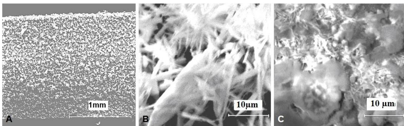
Fig. (4). SEM micrographs of calcium phosphate coatings deposited by the thermal method on a Ti6Al4V substrate at different magnifications.
