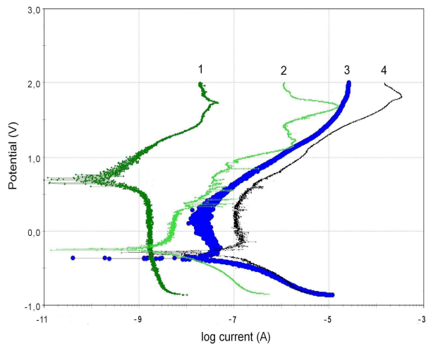
Fig. (7). Anodic polarization curves: 1- Ti6Al4V/Al 2 O 3 , 2- Ti6Al4V/Al 2 O 3 /HAp, 3- Ti6Al4V, 4- Ti6Al4V/HAp samples in SBF solution.
